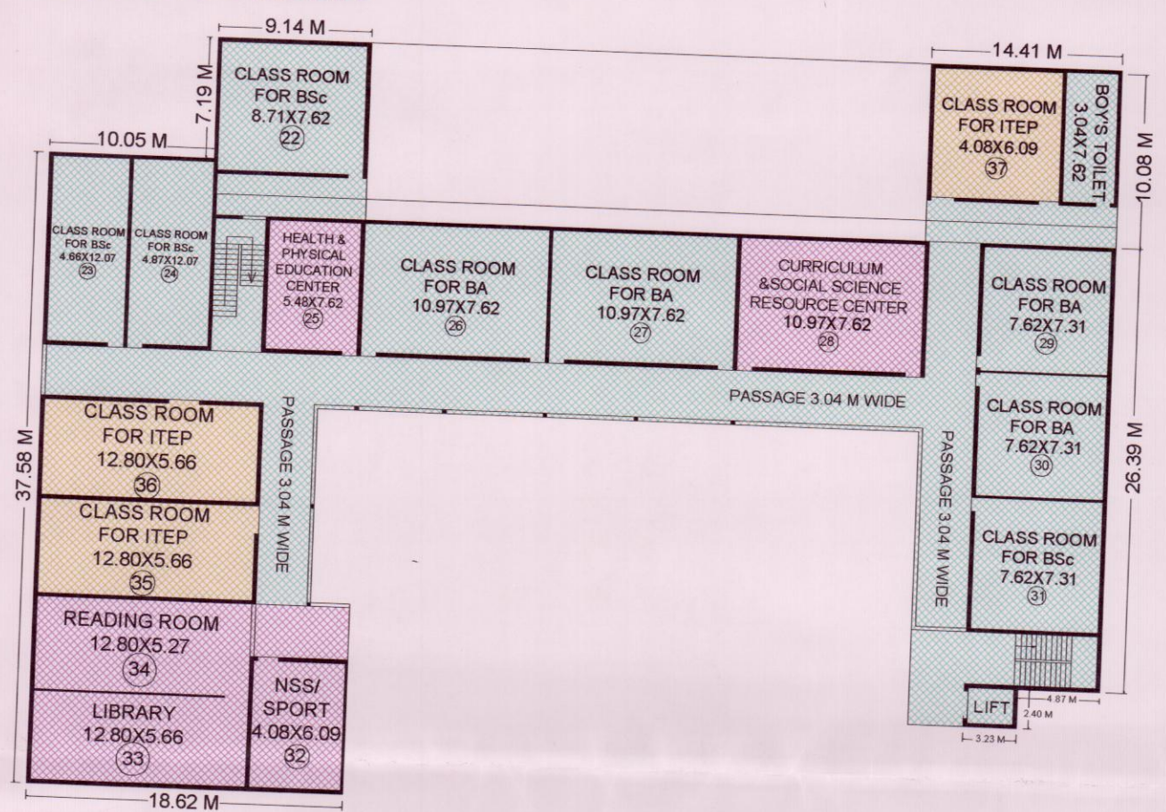
FIRST FLOOR
