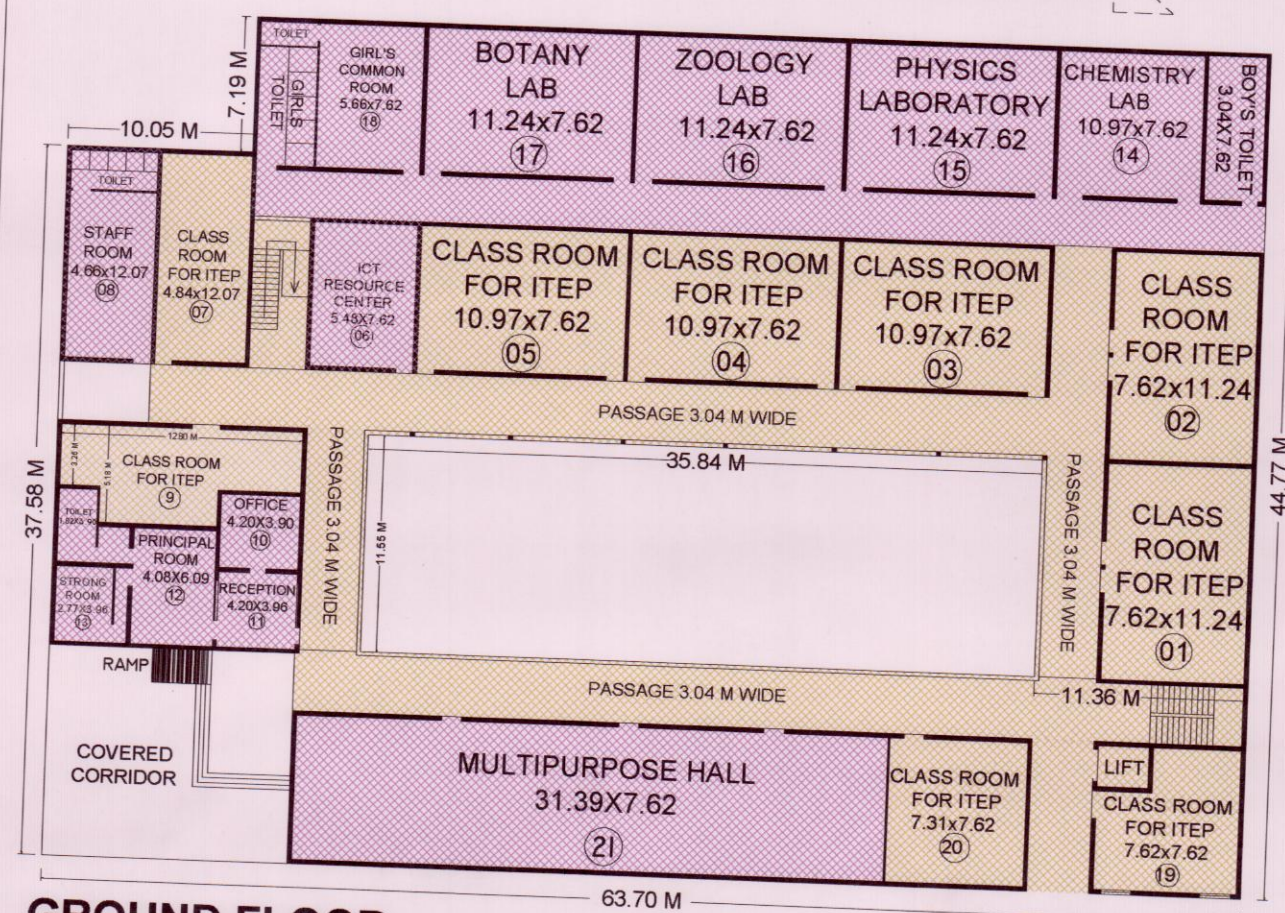
GROUND FLOOR
